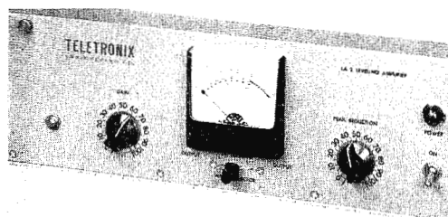
Teletronix LA-2 Leveling Amplifier
