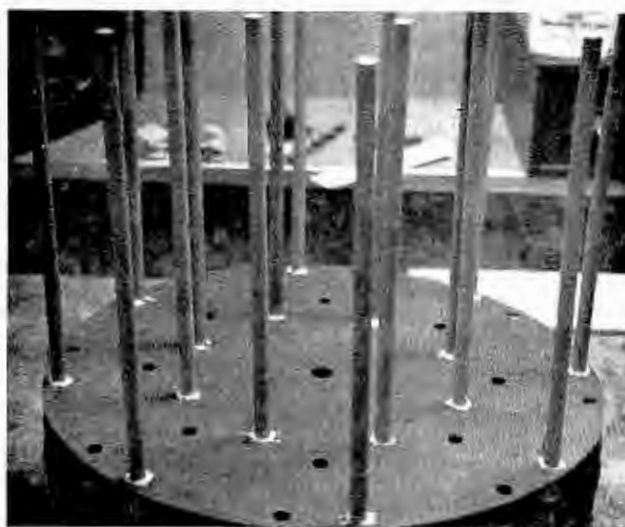
Fig. 2. Construction view showing supporting dowels.
