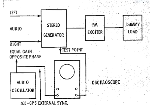
Fig. 7. Test arrangement for stereophonic balance determination steps 3 (a) & 3 (b).
