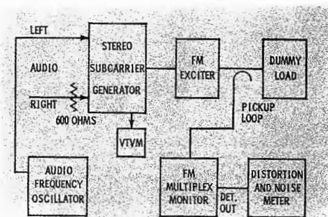
Fig. 3. Diagram of test setup for performing audio response and distortion tests.
