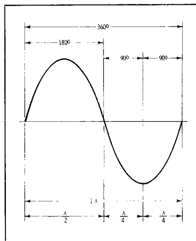
Fig. 2. Degree-wavelength relationship.
