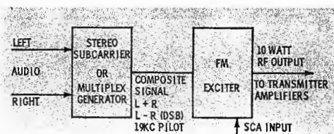
Fig. 2. Diagram of the stereo subcarrier generator and FM exciter, with signals.
