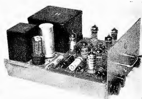
RCA BA-25A AGC Amplifier
